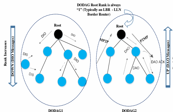
Figure 1. RPL architecture.
