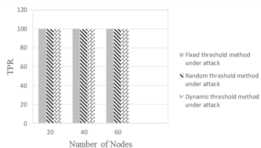
Figure 5. The Detection of DAO Insider Attack
