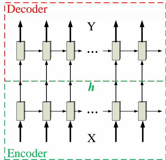
Figure 1. Auto-Encoder-LSTM structur.
