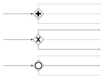
Figure 4. Parallel, Exclusive and Inclusive Gateways, Respectively (Green Arrows Are Executed)
