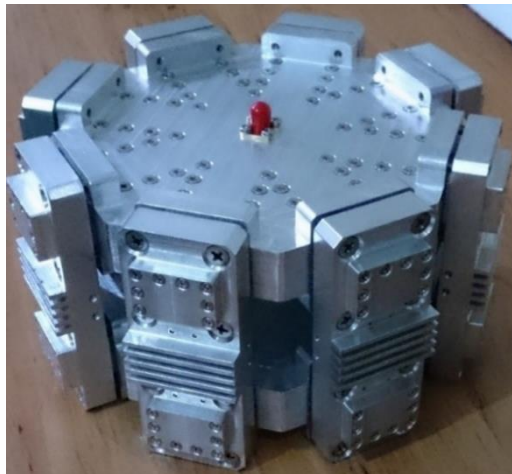
Figure 10. The fabricated radial power combiner in back to back configuration
