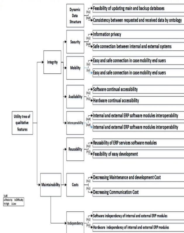
Fig. 3: ATAM utility tree
