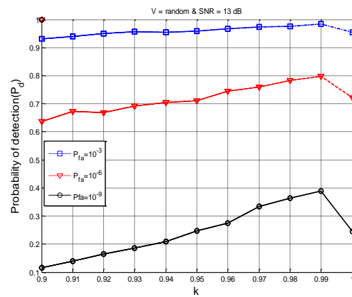
Fig. 7. Probability of detection versus k coefficient for JNAM detector (close view)
