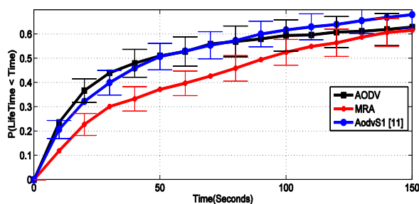
Fig. 4 The CDF of average route life time for AODV, AODVS1[11] and MRA, N = 50 , V_{max} = 15\text{ m/s} , Hello interval = 10 Seconds.
