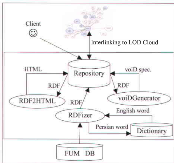
Figure 1. FUM-LD Framework
