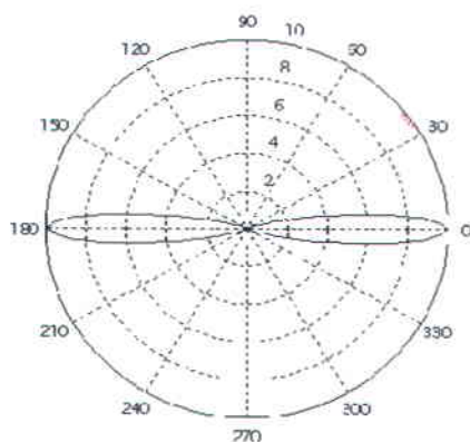
Figure 4. Pattern of directive transmitting antenna
