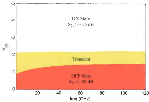
Fig. 9. Defined the ON and OFF region for 600\mu\text{m} TWSW based on the S_{21} (dB).
