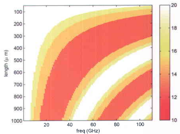
Fig. 17. Division of domain based on S_{11} (OFF).
