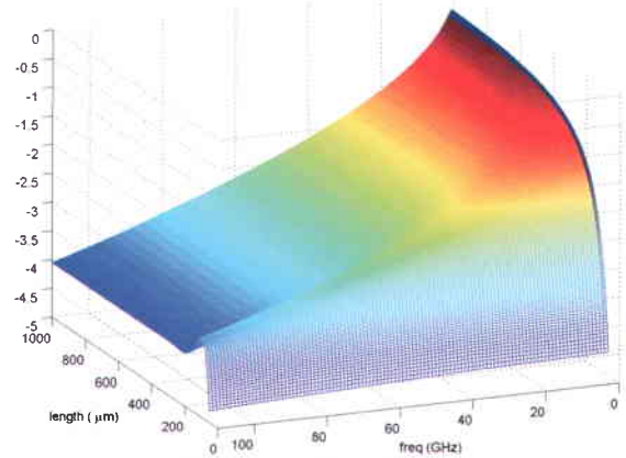
Fig. 12. S_{11} (dB) in OFF state.
