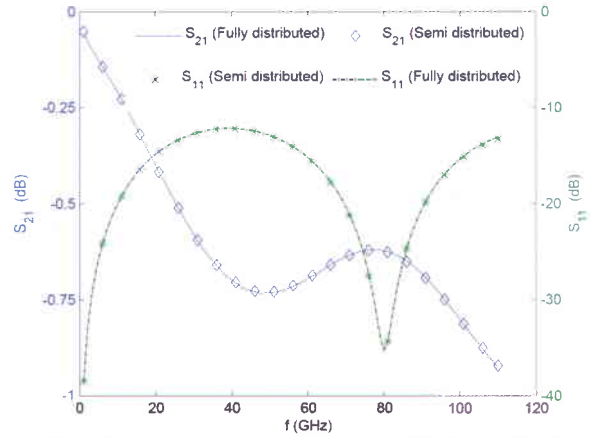
Fig. 10. Calculated insertion loss and reflection coefficient for 600\mu\text{m} TWSW in ON state using scattering parameters and sliced modeling.
