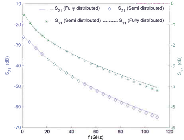
Fig. 11. Calculated isolation and reflection coefficient for 600\mu\text{m} TWSW in OFF state using scattering parameters and semi-distributed modeling.
