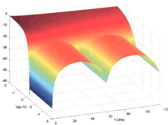
Fig. 8. Calculated S_{11} (dB) for 600\mu\text{m} TWSW in various Control Voltage ( V_{gs} ) and operation frequency.
