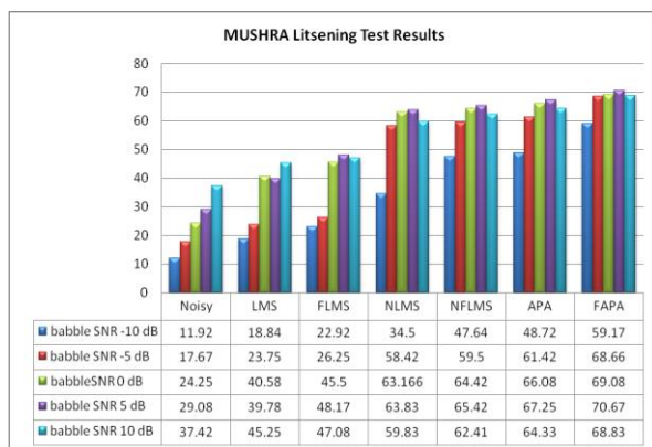
Fig. 10: Averaged MOS results of the enhanced speech obtained by LMS, FLMS, NLMS, NFLMS, APA, and FAPA using babble input noise and 30-order FIR filter as acoustic path under different SNR conditions.
