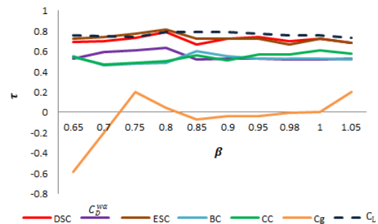
(b) Example network with 23 node
