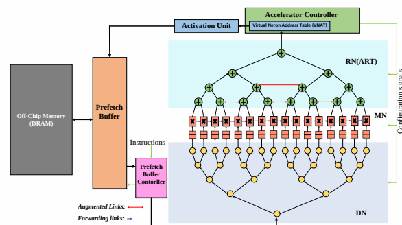
Figure 2. The MAERI accelerator's architecture [11]
