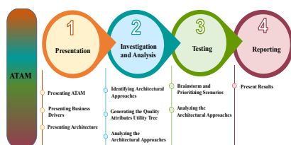
Figure 3. ATAM method
