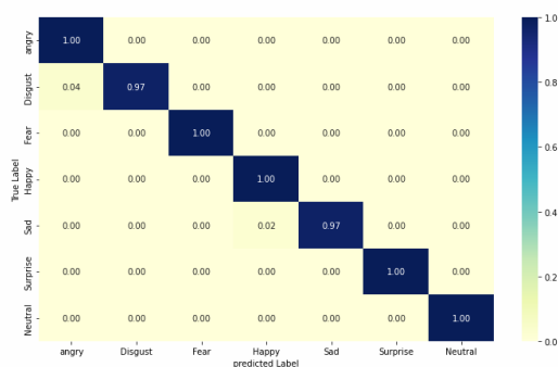
(b) Confusion matrix of CK+
