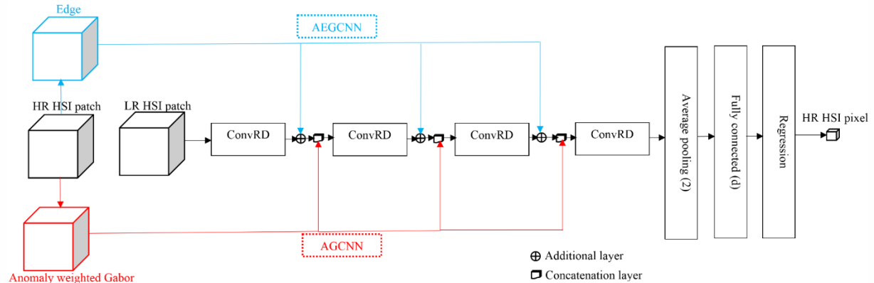
Figure 1. Fig. 1. Blockdiagram of the proposed AGCNN and AEGCNN networks.
