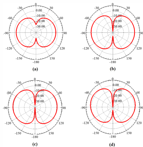
Figure 7. Measured radiation patterns at: (a) 900 MHz, (b) 1800 MHz, (c) 2100 MHz, (d) 2600 MHz for the antenna studied in Fig. 5.
