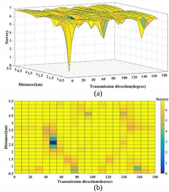
Figure 10. Secrecy rate for SU: (a) Three-Dimensional, (b) Two-Dimensional.
