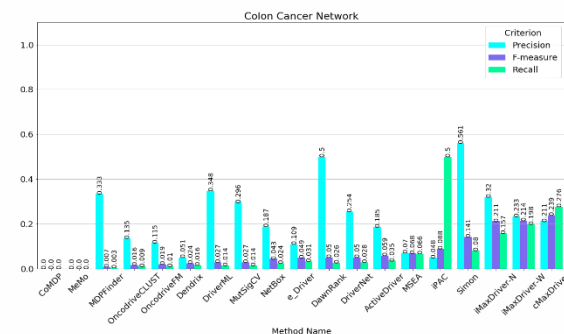
Fig. 7. Comparison of evaluation criteria of the cMaxDriver and other methods in colon cancer.
