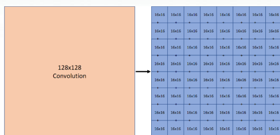
Figure 7. Executing 128x128 convolution in sixty fourth consequent steps.
