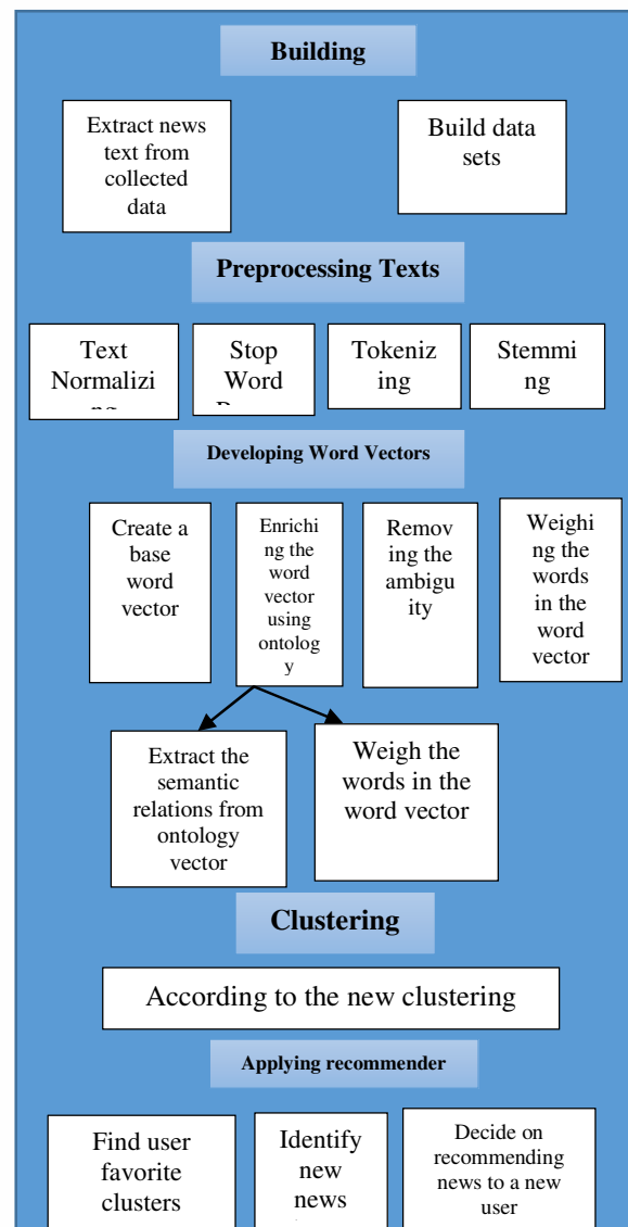
Figure 1. The proposed recommender system.
