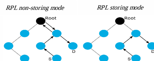
Figure 2. An RPL instance in both storing and non-storing modes.
