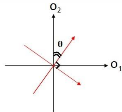
Figure 4. Orthogonalized vectors.
