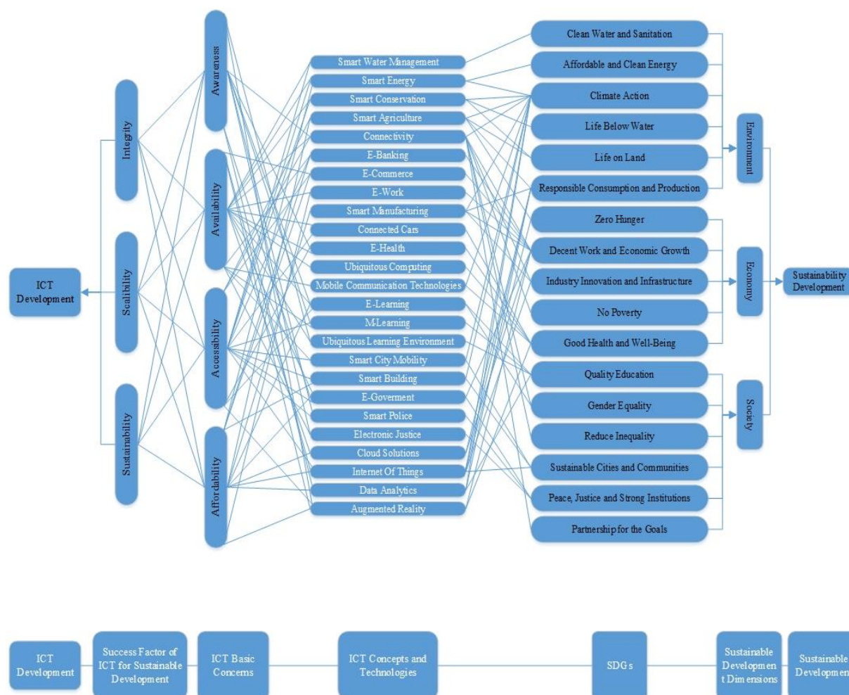
Figure 2. Proposed Framework
