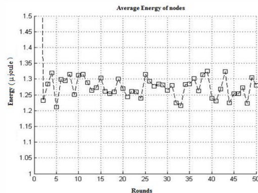
Figure 8. Average energy consumption of the nodes in DISOT during rounds
