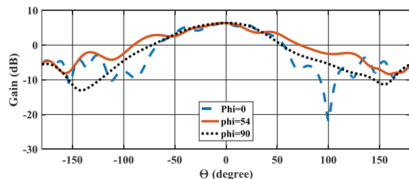
Figure 10. The radiation pattern at the different planes when port 1 is excited.
