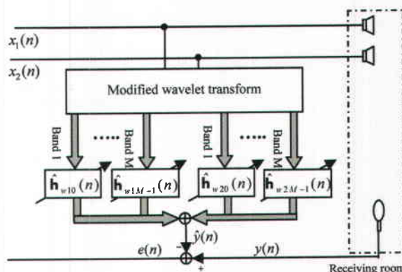
Figure 4. the schematic diagram of proposed structure
