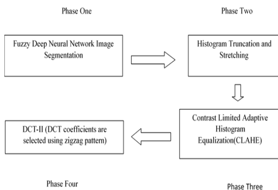
Fig 2. Illumination Normalization Phases
