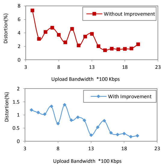
Fig. 19. Distortion as function of peer's uploads bandwidth
