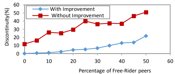
Fig. 22. Discontinuity as function of Free-riders
