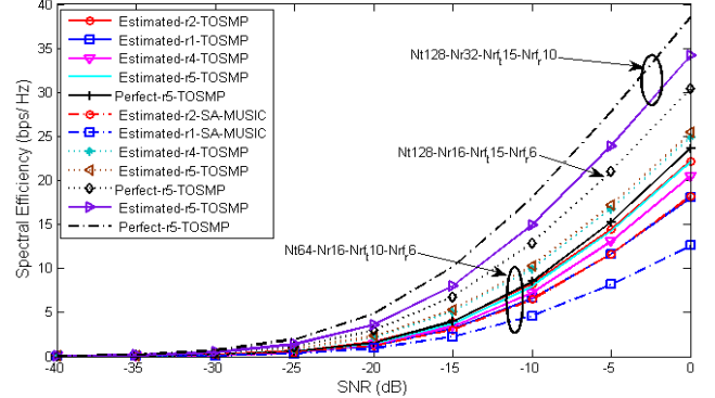
Fig.9 Spectral efficiency versus SNR
