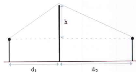
Figure 2. Diffraction geometry
