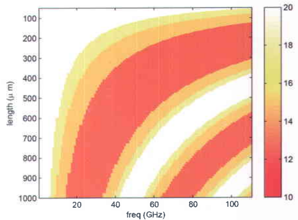
Fig. 17. Division of domain based on S_{11}(\text{OFF}) .
