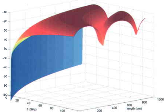
Fig. 15. S_{11} (dB) in ON state.
