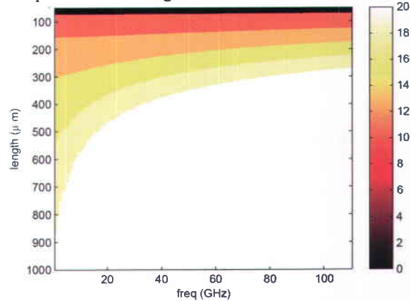
Fig. 16. Division of domain based on S_{21}(\text{OFF}) .
