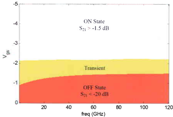
Fig. 9. Defined the ON and OFF region for 600 \mu m TWSW based on the S_{21} (dB).
