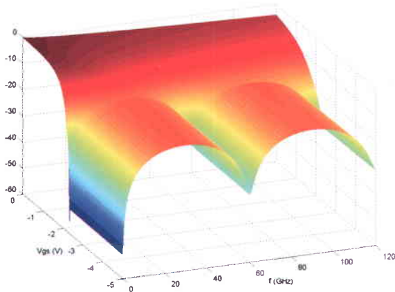
Fig. 8. Calculated S_{11} (dB) for 600 \mu m TWSW in various Control Voltage ( V_{gs} ) and operation frequency.
