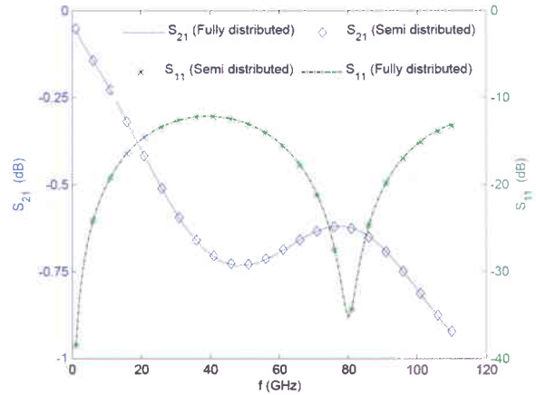
Fig. 10. Calculated insertion loss and reflection coefficient for 600 \mu m TWSW in ON state using scattering parameters and sliced modeling.
