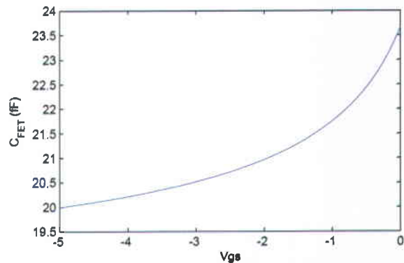
Fig. 6. C_{FET} versus V_{gs} for 100 \mu m TWSW.
