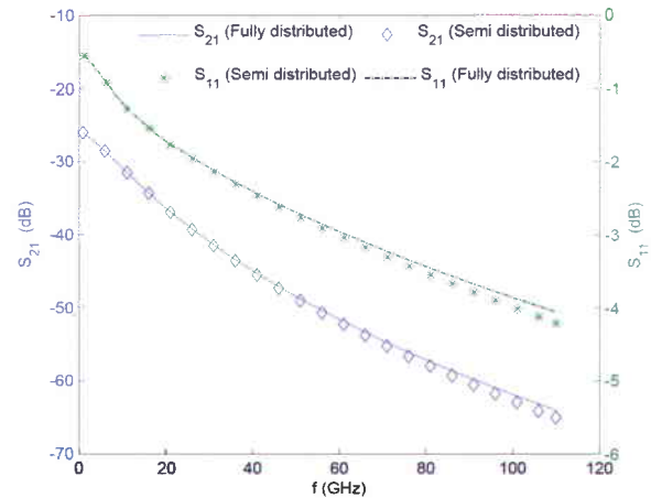
Fig. 11. Calculated isolation and reflection coefficient for 600 \mu m TWSW in OFF state using scattering parameters and semi-distributed modeling.
