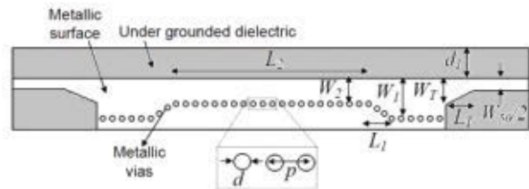
Fig. 2 Configuration of the proposed LWA antenna
