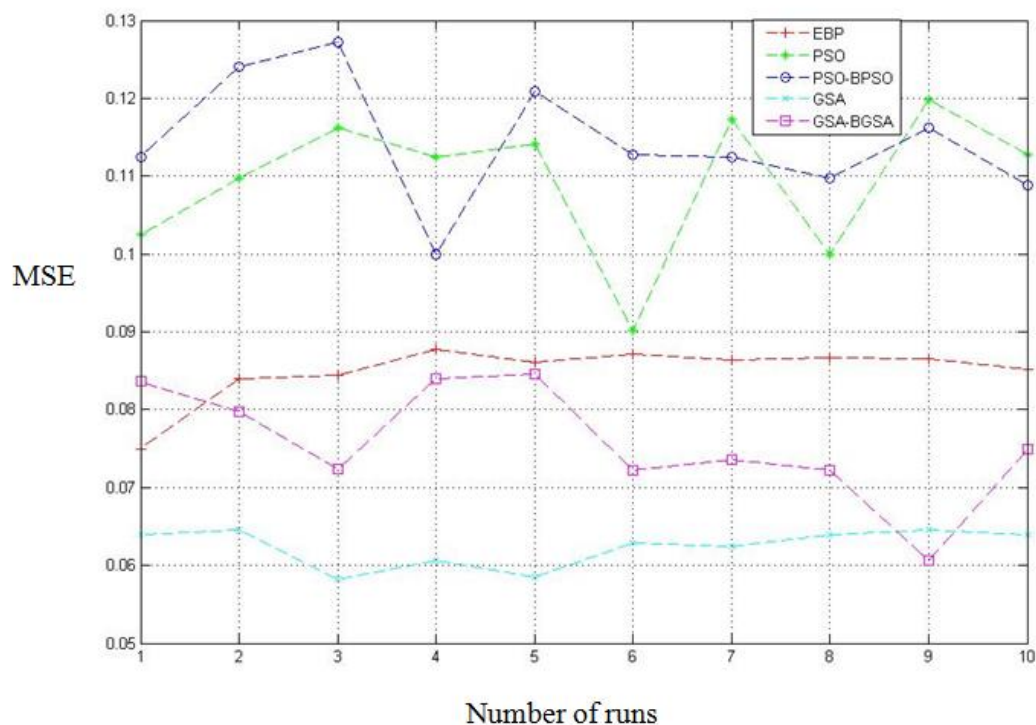
Fig. 3. MSE of the five methods for emotion recognition using 39 input features in 10 runs
