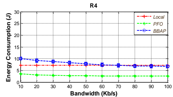
Fig 6. Bandwidth Impact on energy consumption using R4
