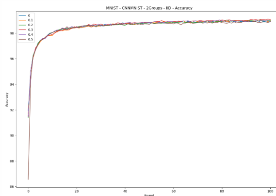
Figure 5. MNIST CNNMNIST IID setup Accuracy
