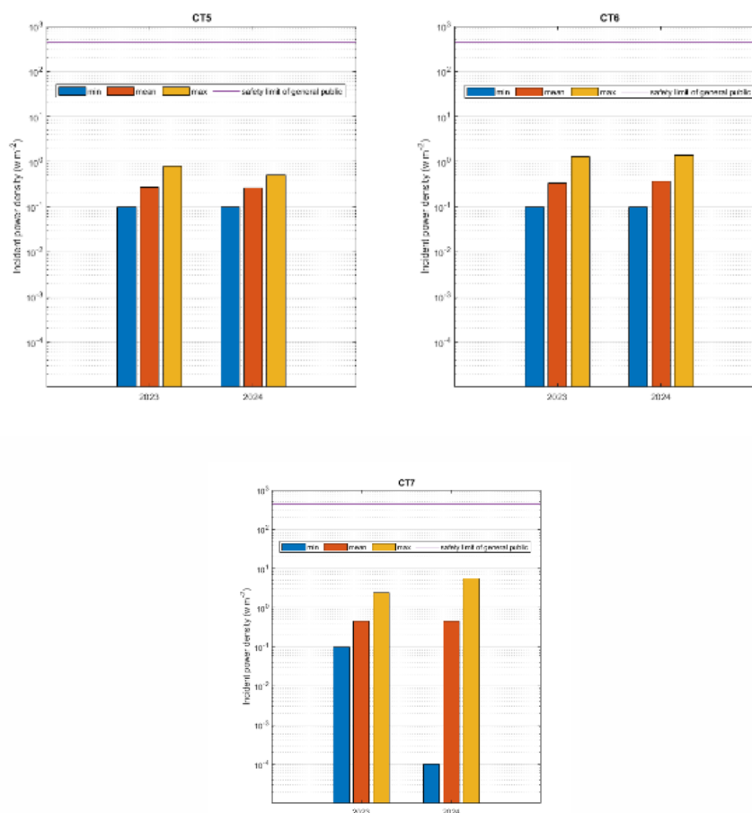
Figure 1. Minimum, mean and maximum value of measured power density the cities according to the data acquisition in 2023 and 2024.
