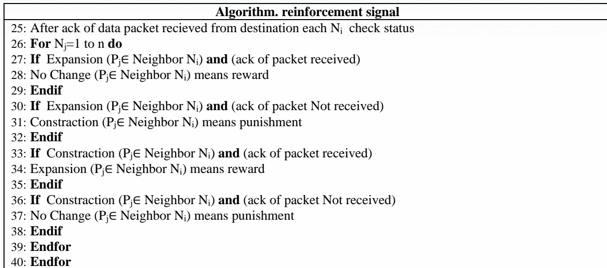
Figure 5. Reinforcement signal in learning phase
